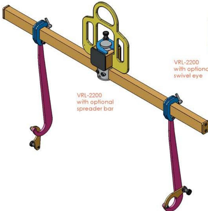
VRL-2200 with examples of lifting accessories.
