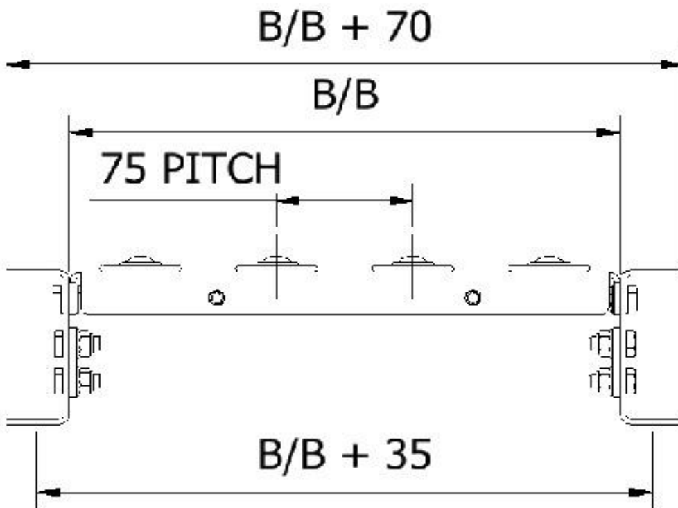
Ball transfer table 750 mm
